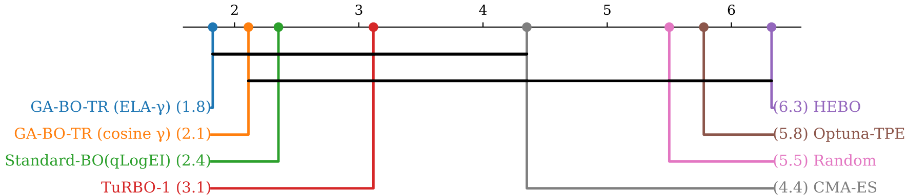
Critical difference (all suites, 21 problems, \alpha=0.05 )
